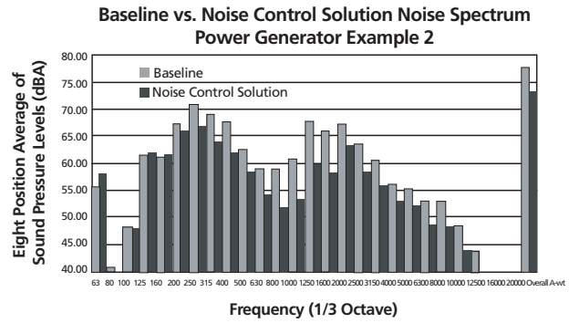
Figure 7: 8 position SPL average for power generator 2 with and without noise control solution
